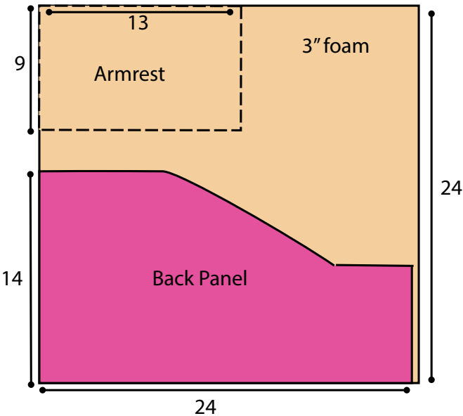
Foam Assembly Diagram I
